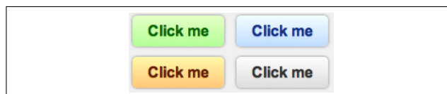
Figure 20. Theme derivation
